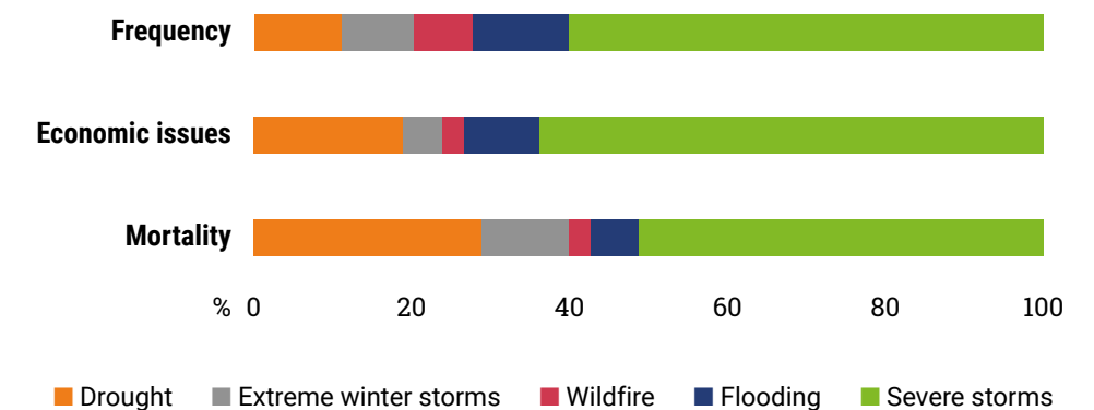
US billion-dollar weather/climate disasters (1980 – mid 2017) 1
